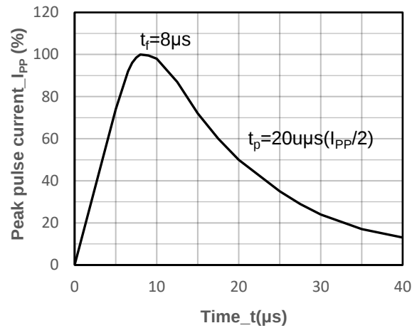
8/20µs Pulse Waveform
