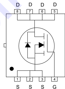
Pin Configuration
